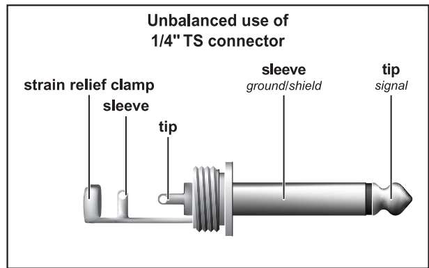
Fig. 3.2: 1/4" mono plug
