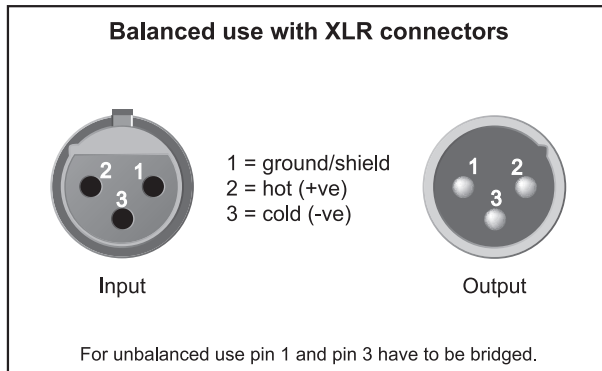
Fig. 3.1: XLR connections
