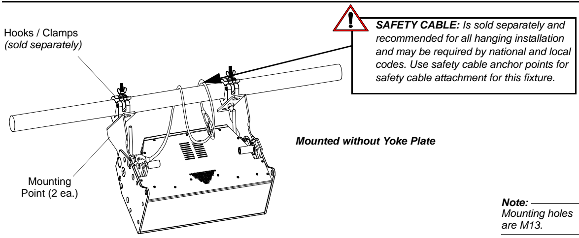
Figure 7: Mounting Luminaire
