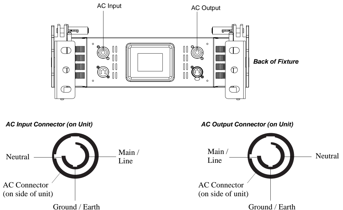
Figure 4: SL NITRO 510C LED STROBE Luminaire AC Input & Output Connections
