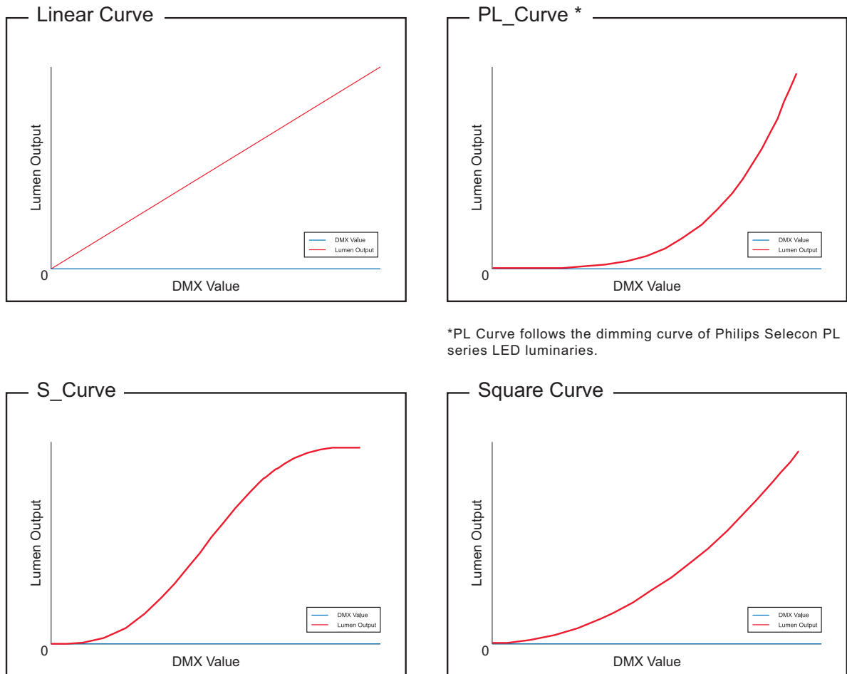
Figure 14: SL NITRO 510C LED STROBE Luminaire Dimmer Curves
