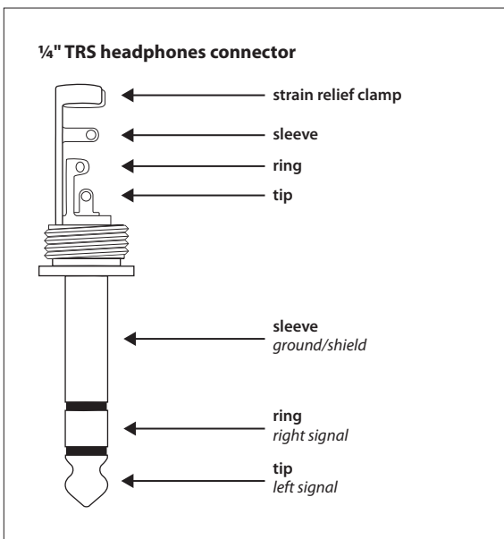
Fig. 4.5: 1/4" TRS connector for headphones
