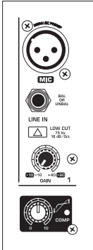
Fig. 2.1: Connectors and controls of mic/line inputs
