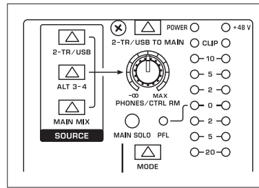
Fig. 2.11: Control room/phones section, level meter
