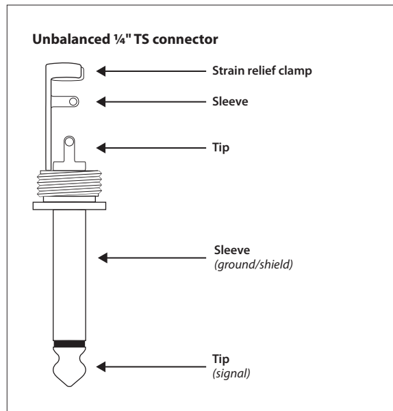
Fig. 4.3: 1/4" TS connector
