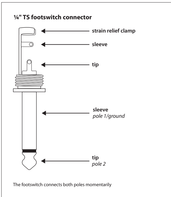
Fig. 4.1: 1/4" TS connector for foot switch
