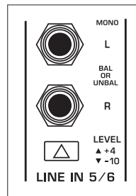
Fig. 2.5: Stereo channel inputs and LEVEL switch
