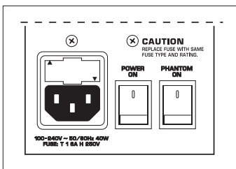
Fig. 2.16: Voltage supply and fuse
