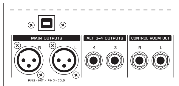
Fig. 2.14: Main mix outputs, Alt 3-4 outputs and control room outputs
