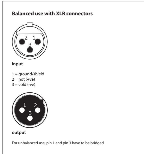
Fig. 4.2: XLR connections
