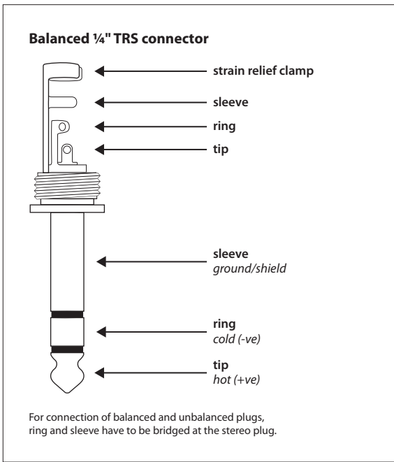
Fig. 4.4: 1/4" TRS connector
