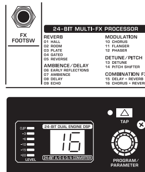
Fig. 3.1: Digital effects module (only X1204USB)
